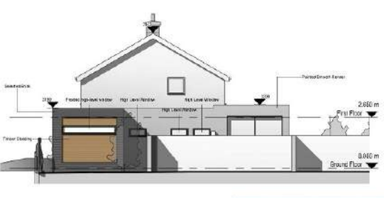
05 Proposed East Elevation 1:100
