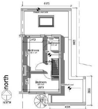
02 Proposed First Floor Plan 1:100
