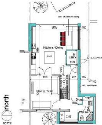
01 Proposed Ground Floor Plan 1:100
