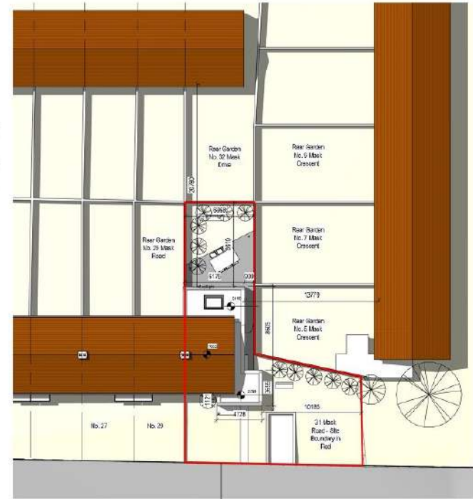
07 Proposed Site 1:200
