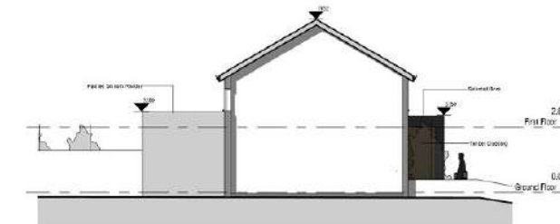
06 Proposed West Elevation 1:100
