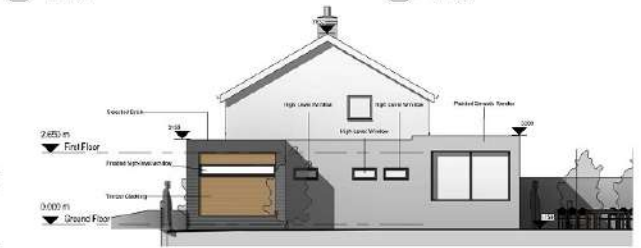
11 Proposed East Elevation (Without Wall) 1:100
